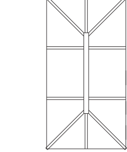
Maximum size Regular lantern as per this rafter layout 3000mm x 4000mm – can go up to 5000mm x 10000mm with additional rafters.
